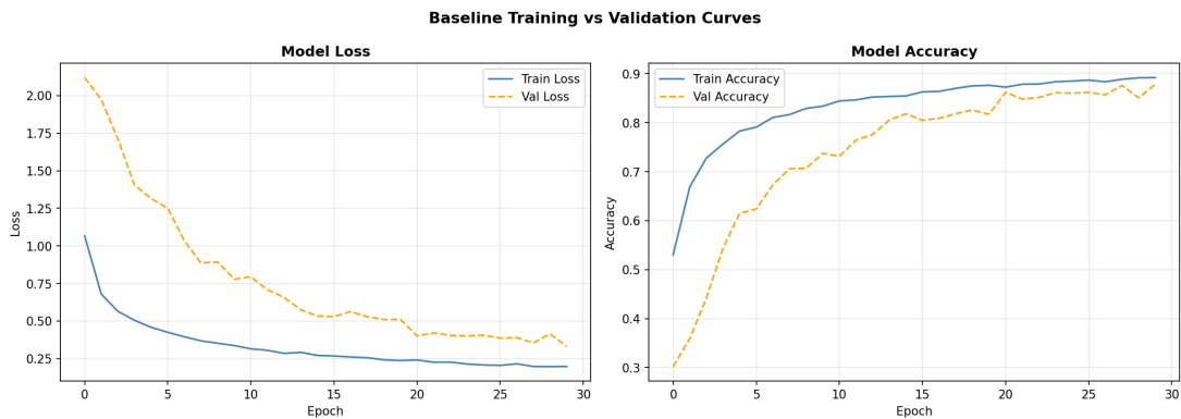
Figure 2: Corrected baseline training and validation loss/accuracy curves
